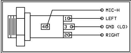
Audio Jack Wiring Detail
